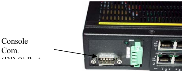
Enlarged view of Magnum 6K16V Console Port area
